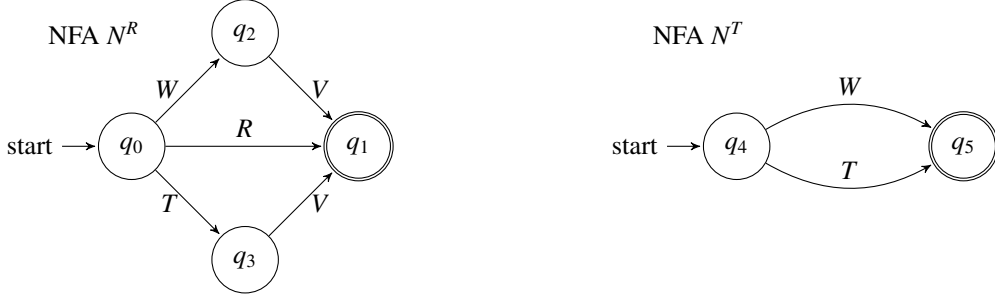
Figure 2: NFAs for predicates R (left) and T (right) from Example 31
